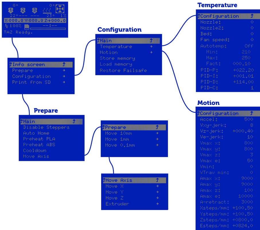
Figure 6.4: Configuration Menu
