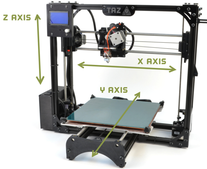
Figure 1.21: Axes movement directions
